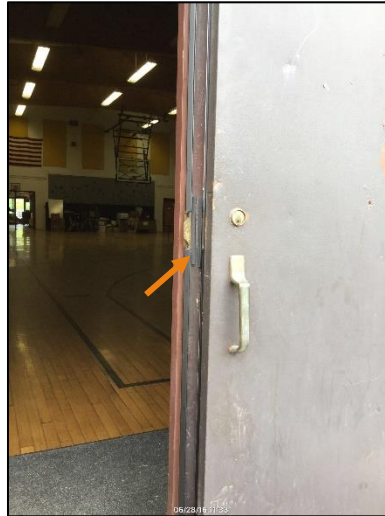
Weather stripping on exterior doors at RDMS and TGS
